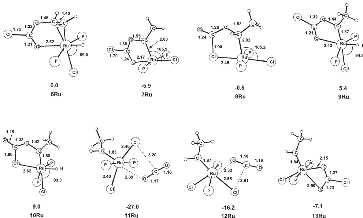
Fig. 4 Detailed geometry (Å and degrees) of species in Fig. 2.
