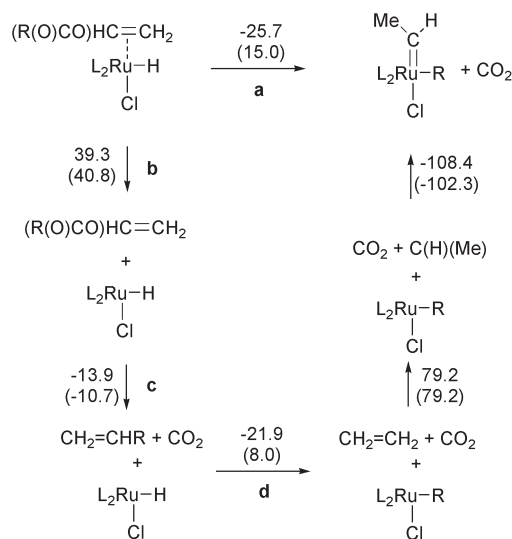
Fig. 6 DFT energies for the reactions shown, contrasting R = Cl with R = CH 3 (in parentheses).
