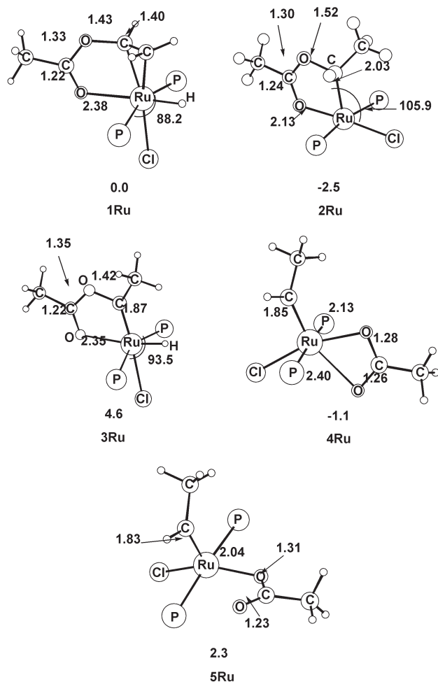
Fig. 3 Detailed geometry ( \text{\AA} and degrees) of species from Fig. 1.
