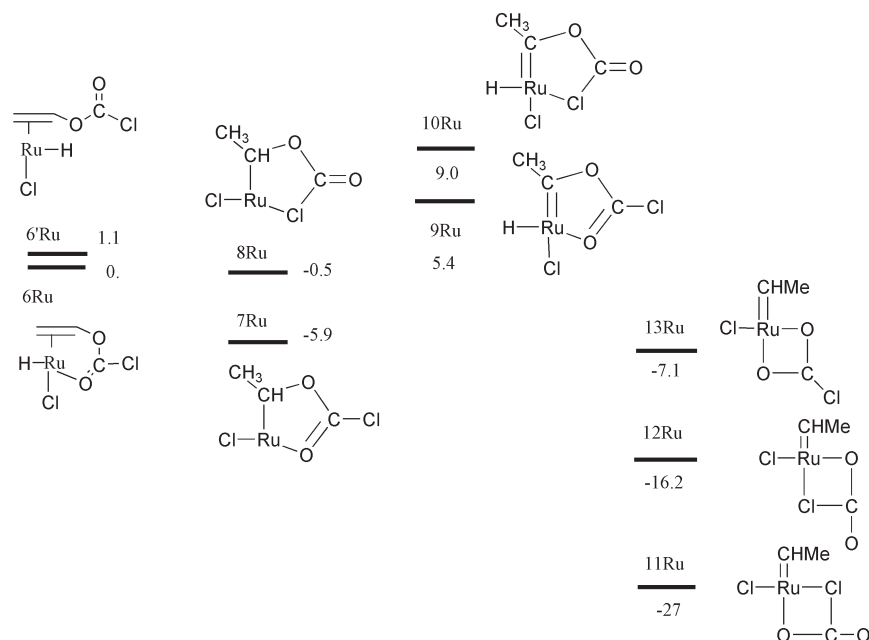
Fig. 2 Calculated (DFT) energies ( \text{kcal mol}^{-1} ) of isomeric structures derived from \text{RuHCl}(\text{PH}_3)_2 and \text{H}_2\text{C}=\text{CH}(\text{O}_2\text{CCl}) . For clarity, the two \text{PH}_3 groups equidistant from the \text{RuHCl} plane are not drawn.
