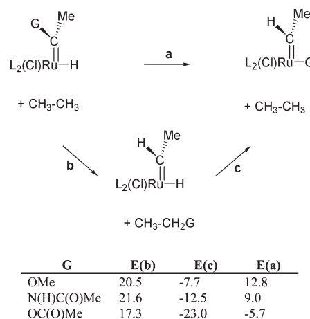
Fig. 5 Thermodynamic cycle and DFT energies for isomerization of variable groups G from carbene carbon to Ru.
