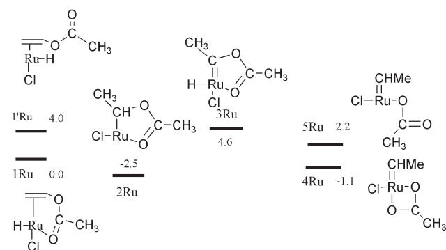
Fig. 1 Calculated (DFT) energies (kcal mol -1 ) of isomeric structures derived from \text{RuHCl}(\text{PH}_3)_2 and \text{H}_2\text{C}=\text{CH}(\text{O}_2\text{CMe}) . For clarity, the two \text{PH}_3 groups equidistant from the \text{RuHCl} plane are not drawn.
